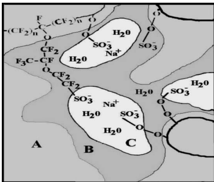
Fig. 13.2 Structure of perfluorosulphonic acid co-polymer (Nafion®). The Yeager Three Phase Model, based on a three-phase clustered system with interconnecting channels within the polymer. (a) Fluorocarbon backbone, (b) interfacial region of relatively large fractional void volume containing some pendant side chains, some water and sulphate groups, (c) clustered regions
