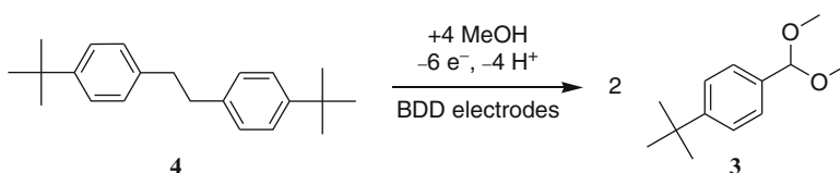
Fig. 5.8 Bond cleavage in 1,2-DPTE in the synthesis of p -tert-butylbenzaldehyde dimethyl acetal ( 3 ). Reagents and conditions: BDDE, 2% 1,2-DPTE, 0.5% H 2 SO 4 (96%), MeOH, 3.4 A dm -2 , 54°C, 8 F mol -1 ; yield = 47% ( 3 )
