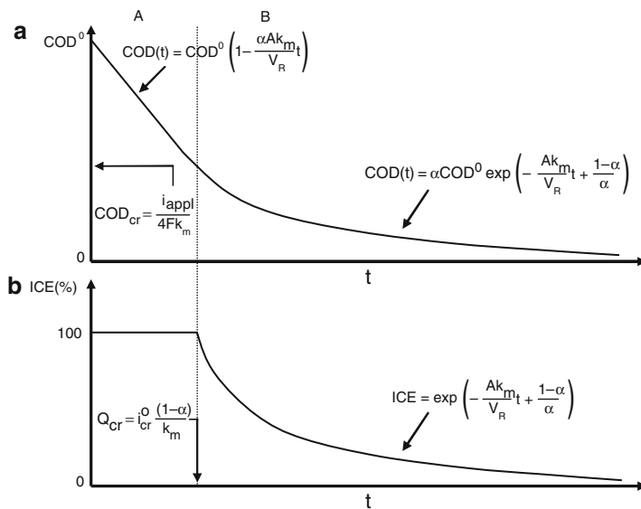
Fig. 1.6 Evolution of (a) COD and (b) ICE in function of time (or specific charge); A represents the charge transport control; B represents the mass transport control
