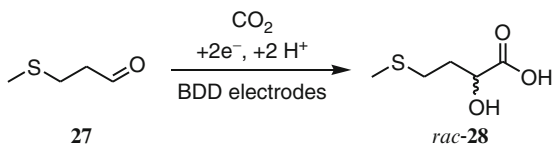
Fig. 5.14 Electrochemical carboxylation of aldehydes. Reagents and conditions: divided flow cell, Nafion ® membrane, BDD/Si electrodes, \text{NBu}_4^+\text{BF}_4^- in DMF, 20–25°C, 0.6 A dm -2 , 5 h, 27% yield in rac - 28 at 88% conversion of 27
