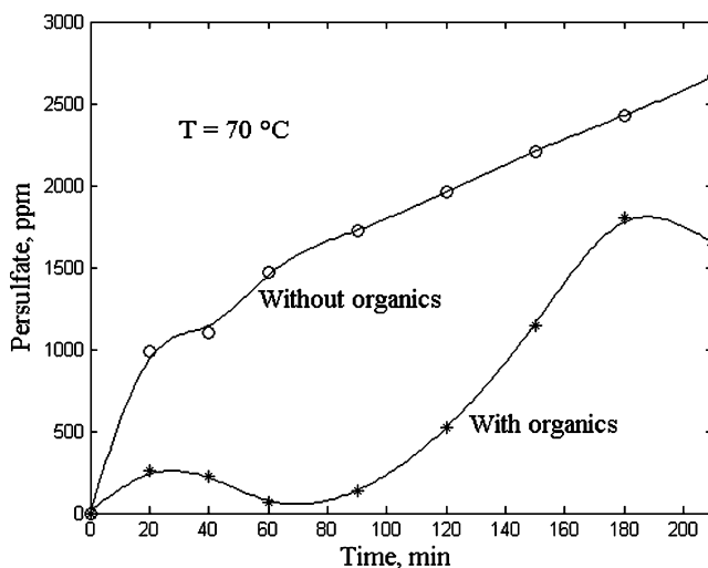
Fig. 9.5 Persulfate concentration vs. treatment time of two solution containing initially sulfuric acid solutions with and without salicylic acid. Initial sulfuric acid concentration 1 \text{ mol dm}^{-3} , initial salicylic acid concentration 3.6 \text{ mmol dm}^{-3} , temperature 70^\circ\text{C} , and applied current density 15.8 \text{ mA cm}^{-2}
