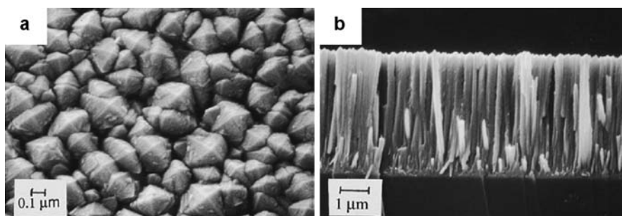
Fig. 18.15 \text{TiO}_2 films deposited by reactive DC magnetron sputtering: (a) Top view and (b) cross-sectional view [reprinted with permission from Weinberger and Garber (1995) , Copyright 1995, American Institute of Physics]
