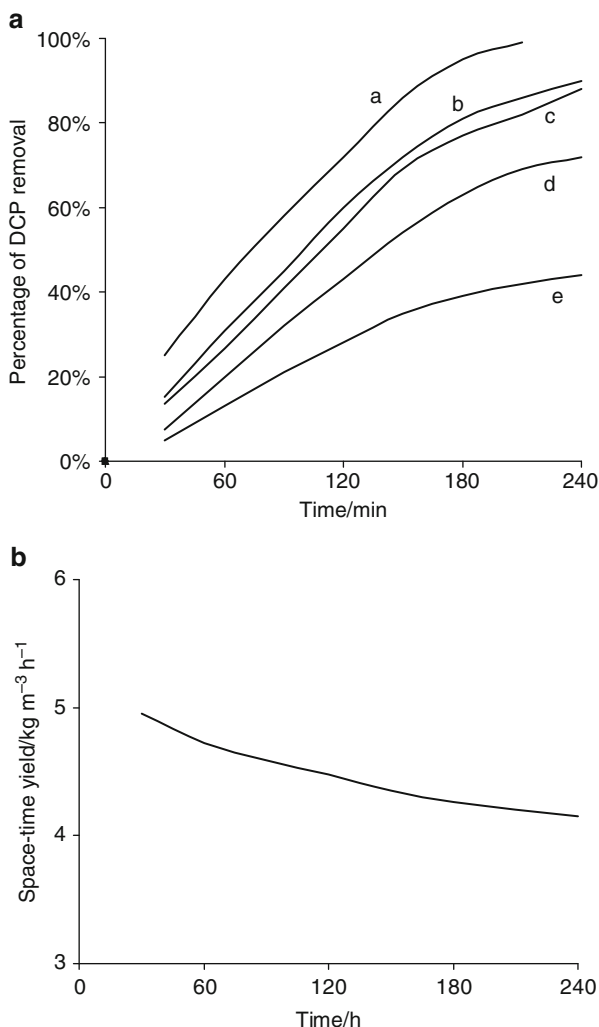
Fig. 13.9 (a) Variations in percentage of 2,4-dichlorophenol (DCP) removal for the electrochemical HDH of DCP in paraffin oil media. Anolyte: 0.5 M H 2 SO 4 aqueous solution (100 cm 3 ). Cathode: Pd/Ti mini-mesh (2 mg Pd cm -2 ). Volume: 100 cm 3 . Curves a: 19.1°C, 5 mM and 10 mA cm -2 ; b: 40°C, 20 mM and 10 mA cm -2 ; c: 19.1°C, 20 mM and 10 mA cm -2 ; d: 19.1°C, 20 mM and 20 mA cm -2 ; e: 19.1°C, 20 mM and 5 mA cm -2 . Other conditions are as in Fig. 13.6. (b) Variations in space-time yield for the electrochemical HDH of DCP in paraffin oil media. Anolyte: 0.5 M H 2 SO 4 aqueous solution (100 cm 3 ). Cathode: Pd/Ti mini-mesh (2 mg Pd cm -2 ). Data were collected at 19.1°C and 10 mA cm -2 in a catholyte of 20 mM DCP in paraffin oil (100 cm 3 ). Other conditions are as in Fig. 13.6
