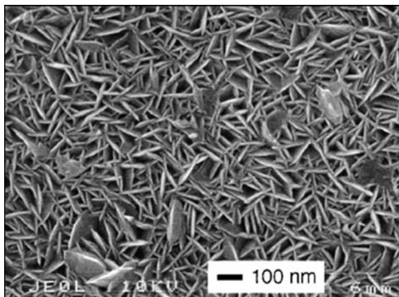
Fig. 18.14 \text{TiO}_2 film deposited by spray-pyrolysis method using \text{TiCl}_4 /titanium isopropoxide as the precursor [reprinted from Okuya et al. (1999), copyright 1999, with permission from Elsevier]
