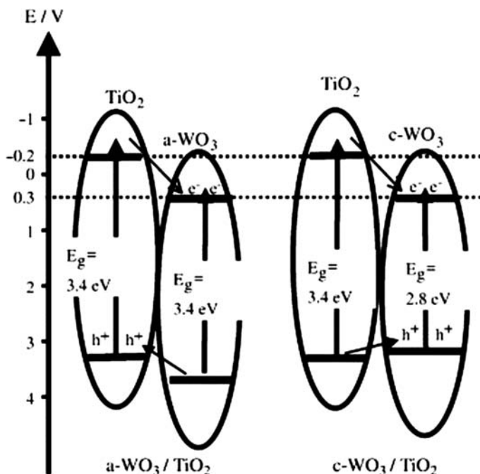
Fig. 16.11 Energetic diagram of amorphous- and crystalline- \text{WO}_3/\text{TiO}_2 [Reprinted from Higashimoto et al. (2006), Copyright (2006), with permission from Elsevier]
