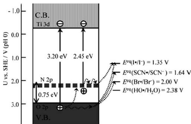
Fig. 16.29 Band structure of N-doped \text{TiO}_2 with the oxidation potentials of a few redox couples [Reprinted with permission from Nakamura et al. (2004). Copyright (2004) American Chemical Society]
