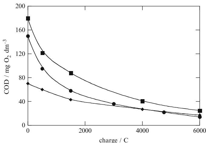
Fig. 19.8 Chemical oxygen demand evolution of O 2 -saturated (filled square) 0.32 mM malathion, (filled circle) 0.50 mM TEPP (tetraethyl-pyrophosphate), and (filled diamond) 0.09 mM parathion ethyl solutions with 2 mM Fe 3+ in 10 -2 M H 2 SO 4 at room temperature in the cathodic compartment of a divided Pt/carbon felt cell at E_{cat} = -0.55 V vs. SCE [adapted from Guivarch et al. (2003a)]
