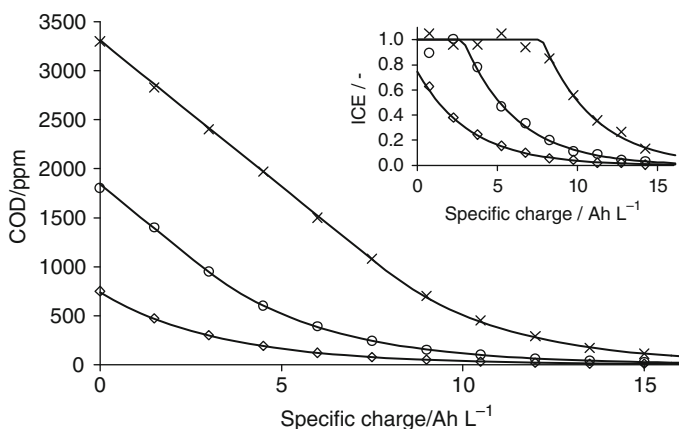
Fig. 1.8 Influence of the initial 2-naphtol concentration: (cross) 9 mM, (open circle) 5 mM, (open diamond) 2 mM on the evolution of COD and ICE (inset) during electrolysis on BDD; i = 238 \text{ A m}^{-2} ; T = 25^\circ\text{C} ; Electrolyte: 1 M \text{H}_2\text{SO}_4 . The solid line represents model prediction
