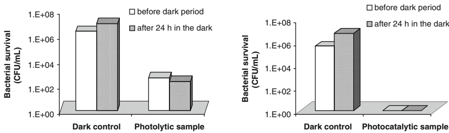
Fig. 17.9 Durability of solar disinfection without catalyst experiment of Fig. 17.7a, September 25th (a). Durability of solar disinfection with catalyst experiment of September 27th, 2003 (b). Initial and final samples were incubated for 24 h in the dark
