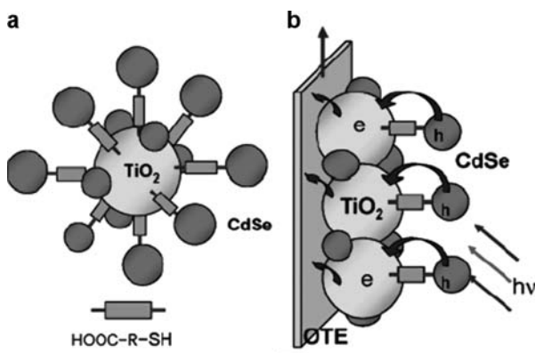
Fig. 16.18 \text{TiO}_2/\text{CdSe} couple linked by organic molecules: (a) particle–particle; (b) particle–film [Reprinted with permission from Robel et al. (2006). Copyright (2006) American Chemical Society]
