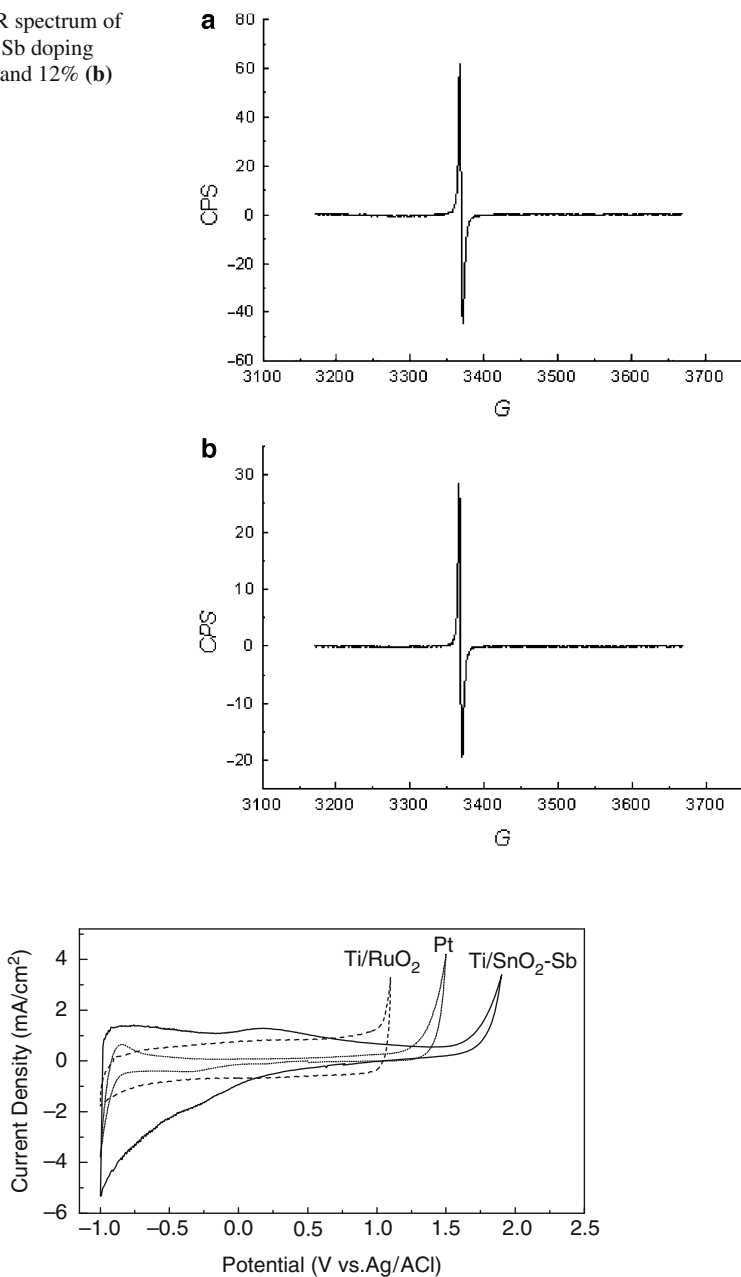
Fig. 14.17 Comparison of cyclic voltammograms of several electrodes in 0.25 \text{ mol L}^{-1} \text{ Na}_2\text{SO}_4 solution
