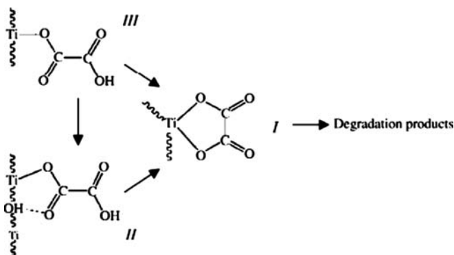
Fig. 16.8 Schematic evolution of the surface composition of oxalates chemisorbed on \text{TiO}_2 surface during UV illumination [Reprinted from Mendive et al. (2005), Copyright (2005), with permission from Elsevier]
