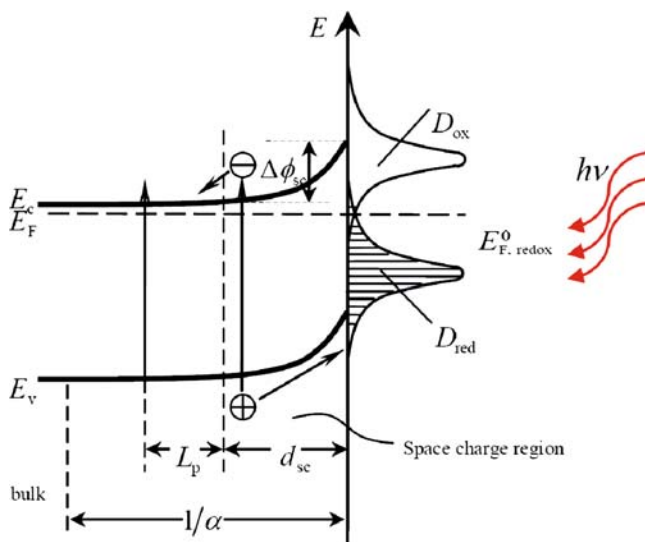
Fig. 16.4 Charge transfer at the n-type semiconductor–solution interface under illumination [Copyright Wiley-VCH Verlag GmbH & Co. KGaA. Reproduced with permission from Memming (2001)]
