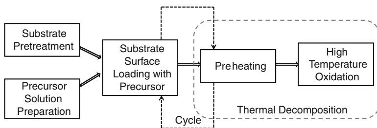
Fig. 3.1 Schematic diagram of thermal decomposition method for making DSA type electrodes
