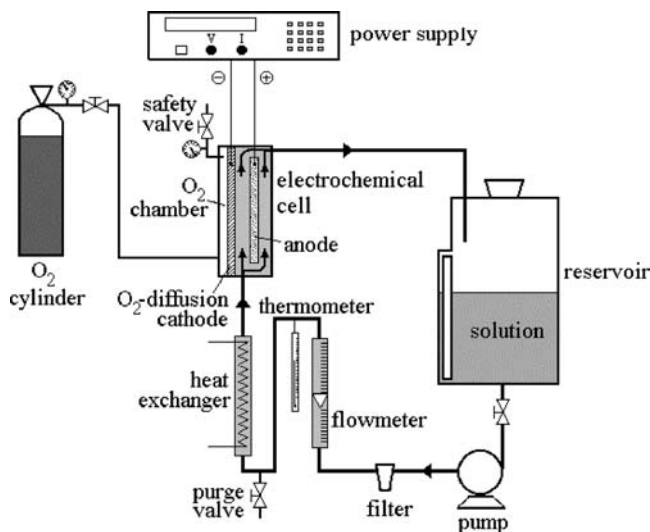
Fig. 19.19 Sketch of the flow plant with an undivided filter-press two-electrode electrochemical reactor fed with oxygen used for the degradation of 30 dm 3 of aniline solutions by electro-Fenton and peroxi-coagulation (Brillas et al. 2002)
