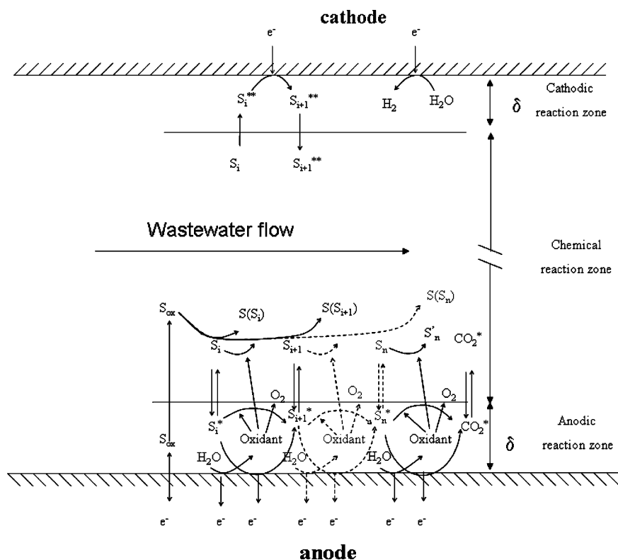
Fig. 4.3 Electrooxidation with active electrodes
