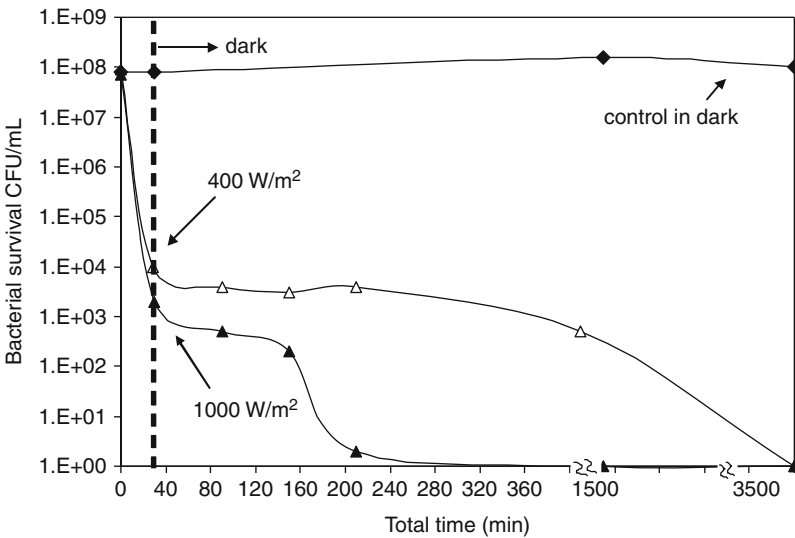
Fig. 17.6 Continuous irradiation of E. coli during 30 min in solar simulator, at 400 and 1,000 \text{ W m}^{-2} . Durability of disinfection in the dark (24 and 60 h). V_{\text{TOT}} = 40 \text{ mL} , \text{TiO}_2 = 0.5 \text{ g L}^{-1} , deionized water. Black dotted line signifies commencement of dark incubation
