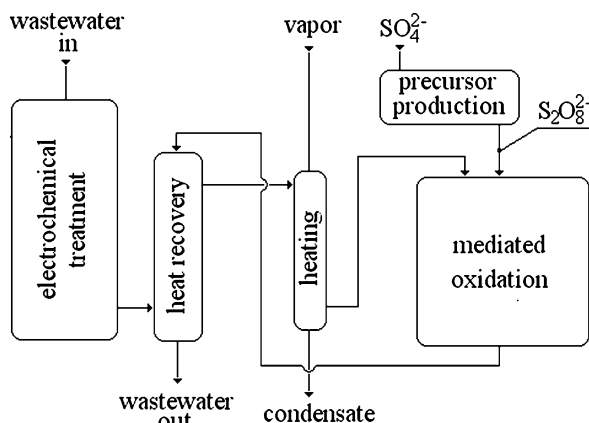
Fig. 9.6 Scheme of wastewater treatment with an initial electrochemical treatment with BDD anodes and a successive two-step mediated oxidation, with the precursor produced locally with the use of the same kind of anodes
