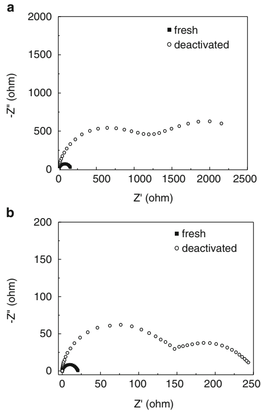
Fig. 14.20 Comparison of electrochemical impedance spectra of freshly prepared electrodes and after accelerated life test in 0.5 mol L -1 H 2 SO 4 solution (a) and in 1.0 mol L -1 NaOH solution (b)
