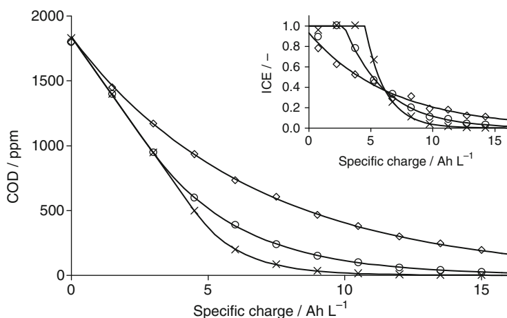
Fig. 1.9 Influence of the applied current density: (cross) 119 \text{ A m}^{-2} , (open circle) 238 \text{ A m}^{-2} , (open diamond) 476 \text{ A m}^{-2} on the evolution of COD and ICE (inset) during electrolysis of 5 mM 2-naphtol in 1 M \text{H}_2\text{SO}_4 on BDD; T = 25^\circ\text{C} . The solid line represents model prediction
