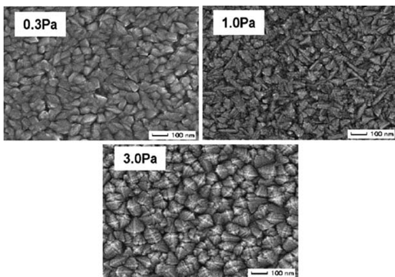
Fig. 18.16 \text{TiO}_2 thin films deposited by RF magnetron sputtering under various pressure [reprinted from Yamagishi et al. (2003) , copyright 2003, with permission from Elsevier]
