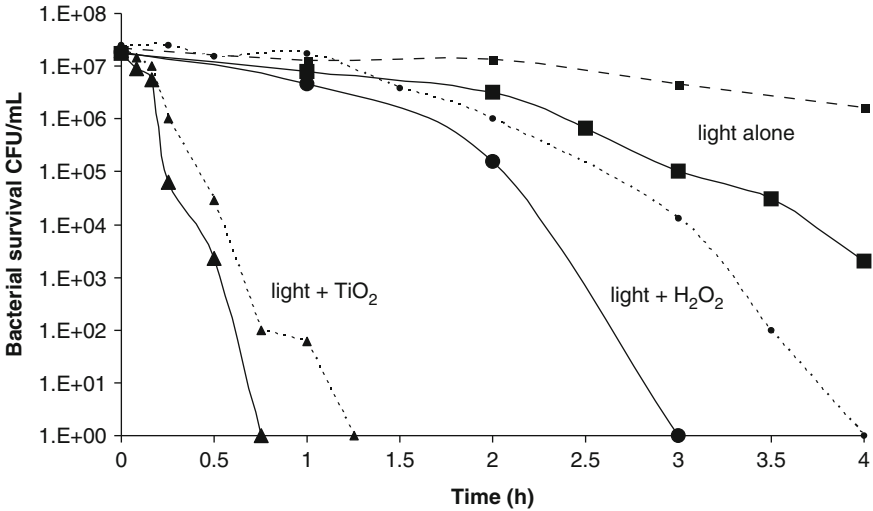
Fig. 17.5 Influence of the generation of E.coli K 12 on light inactivation of bacteria for the systems with (filled triangle) and without (filled square) \text{TiO}_2 addition. System with \text{H}_2\text{O}_2 addition (filled circle). Third generation (dashed line), seven generation (continuous line). \text{TiO}_2 ( 1 \text{ g L}^{-1} ), \text{H}_2\text{O}_2 ( 10 \text{ mg L}^{-1} ). Sun Simulated lamp
