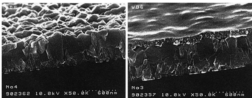
Fig. 16.13 \text{SnO}_2 and \text{TiO}_2/\text{SnO}_2 deposited on glass substrate (Hattori et al. 2000) (Reproduced by permission of The Electrochemical Society)
