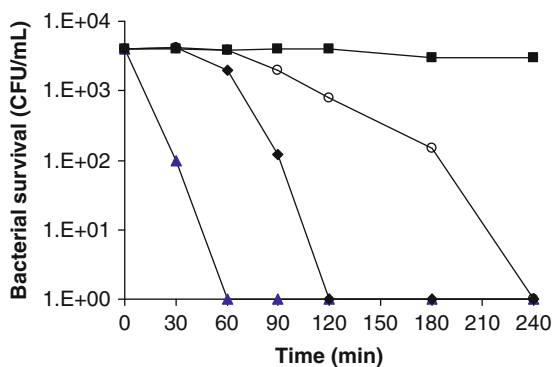
Fig. 17.4 E. coli survival with TiO 2 P25 fixed on NW10 (filled diamond), without TiO 2 (open circle) as a function of time. Suspended TiO 2 (filled triangle). Dark control with fixed TiO 2 0.2\text{ g L}^{-1} (filled square). Caphore system
