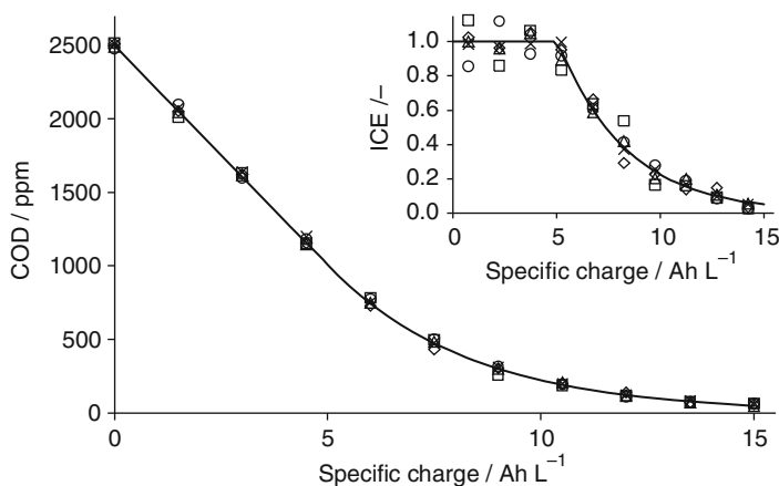
Fig. 1.7 Evolution of COD and ICE ( inset ) in function of specific charge for different organic compounds: ( cross ) acetic acid, ( open square ) isopropanol, ( open circle ) phenol, ( open triangle ) 4-chlorophenol, ( open diamond ) 2-naphtol; i = 238 \text{ A m}^{-2} ; T = 25^\circ\text{C} ; Electrolyte: 1 \text{ M H}_2\text{SO}_4 . The solid line represents model prediction
