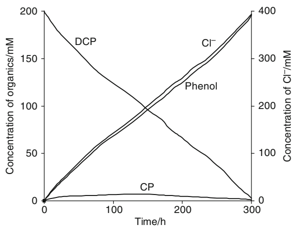
Fig. 13.11 Variations in concentrations during the electrochemical HDH of DCP in paraffin oil media. Catholyte: 200 mM DCP in paraffin oil ( 1,000 \text{ cm}^3 ). Other conditions are as in Fig. 13.7
