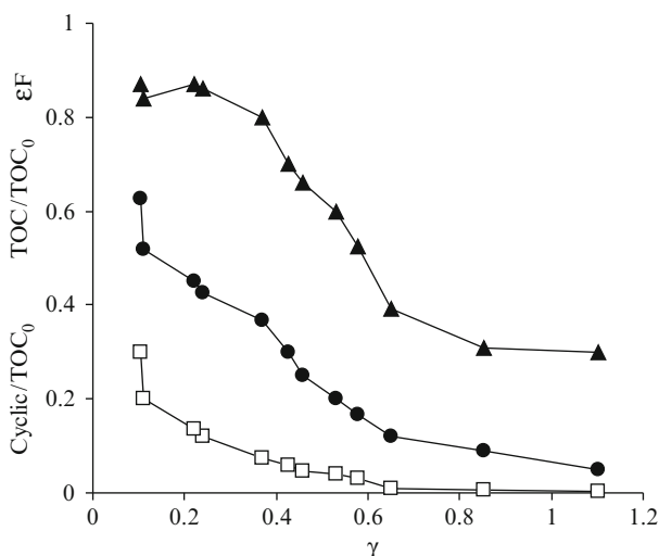
Fig. 8.3 Trend of TOC ( circles ), dissolved carbon attributable to cyclic intermediates ( squares ), both normalised with respect to TOC 0 , and faradic yield ( triangles ) as a function of \gamma
