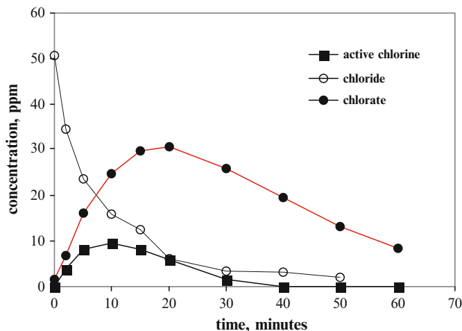
Fig. 7.7 Concentration of chloride, active chlorine and chlorate in discontinuous electrolysis using rotating BDD anode ( \text{IrO}_2 cathode, 200 \text{ A m}^{-2} , 100 mL, 300 rpm, 20^\circ\text{C} , 50 ppm chloride as NaCl)
