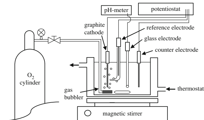
Fig. 19.5 Scheme of an undivided electrolytic cell fed with oxygen to electrogenerate \text{H}_2\text{O}_2 for the treatment of wastewaters [adapted from Panizza et al. (2001)]
