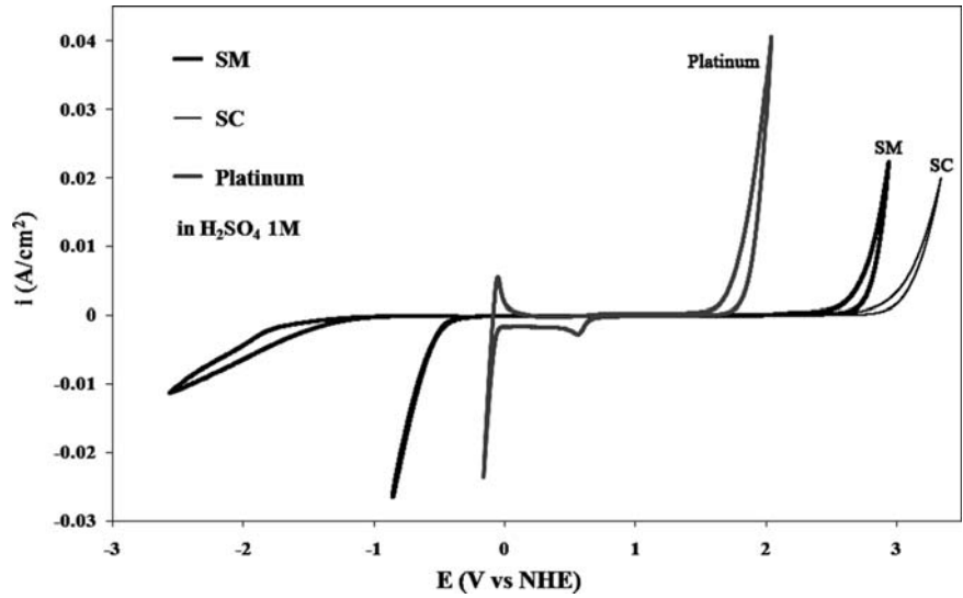
Fig. 6.3 SC (semi-conductor) and SM (semi-metal) BDD electrochemical window compared to that of platinum
