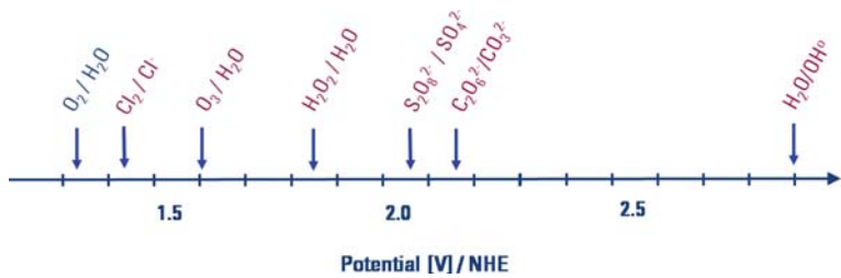
Fig. 6.4 Voltage scale and generated oxidizing species
