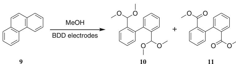
Fig. 5.7 Bond cleavage in phenanthrene to 1,1'-difunctionalized biaryls. Reagents and conditions: BDDE, 2% phenanthrene, 0.5% H 2 SO 4 (96%), 3.4 A dm -2 , 54°C, 10 F mol -1 ; yield = 15% ( 10 ), 39% ( 11 )
